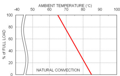
DFEC60-48S05 Derating Curve
