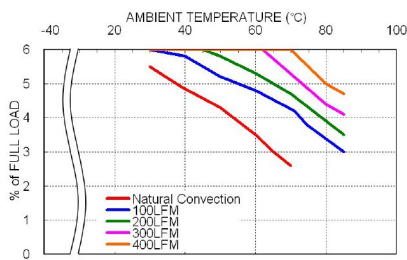
DOS06-12T, Vout=3.3V Derating Curve
