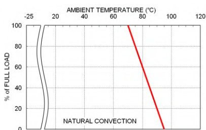
FKC05-48S05 Derating Curve
