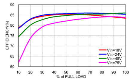
MOP10-48S05WA Efficiency vs. Output Load
