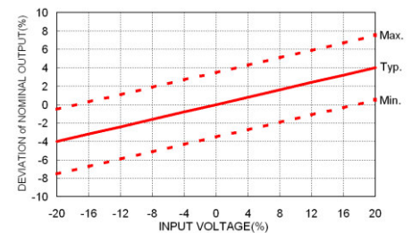
Vout Deviation vs. Input Voltage for 12, 15, 24Vin Models
