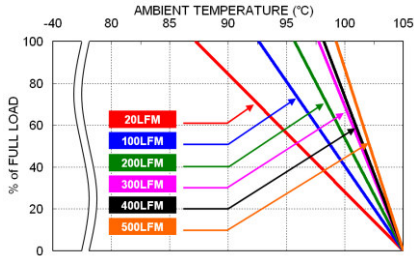
RHK06-110S12W Derating Curve
