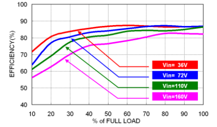
RHK06-110S12W Efficiency vs. Output Load
