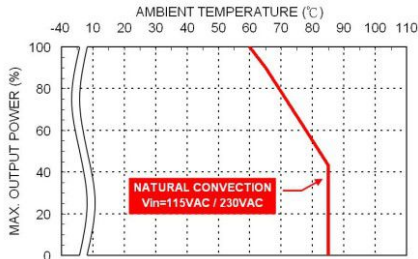
Derating Curve vs. Ambient Temperature TAD30USxxB xx=3P3/05/7P5/09/121/151/18 Connector Option : (□):JST)
