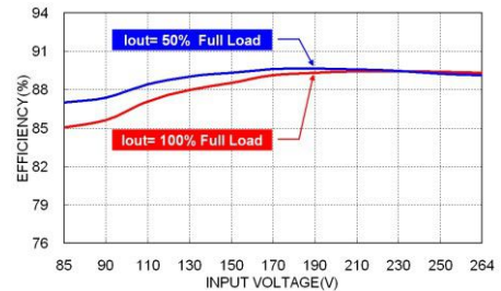
TAD30US24B Efficiency vs. Input Voltage
