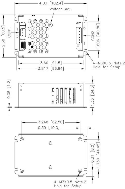
BOTTOM VIEW
