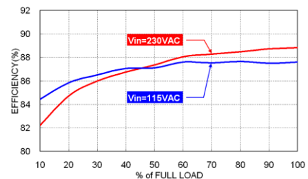
TAD40UT63M6B Efficiency vs. Output Load
