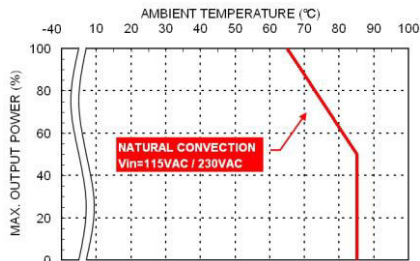
TAD40UD Derating Curve vs. Ambient Temperature
