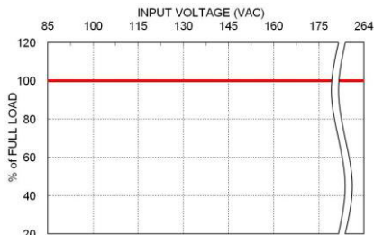
TAD40 Derating Curve vs. Input Voltage
