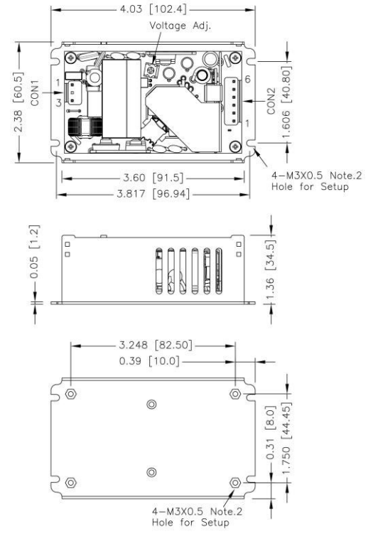
BOTTOM VIEW
