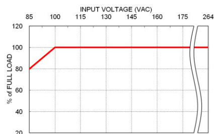
TI-F150 Derating Curve vs. Input Voltage
