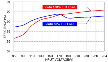
TAF150US24B Efficiency vs. Input Voltage
